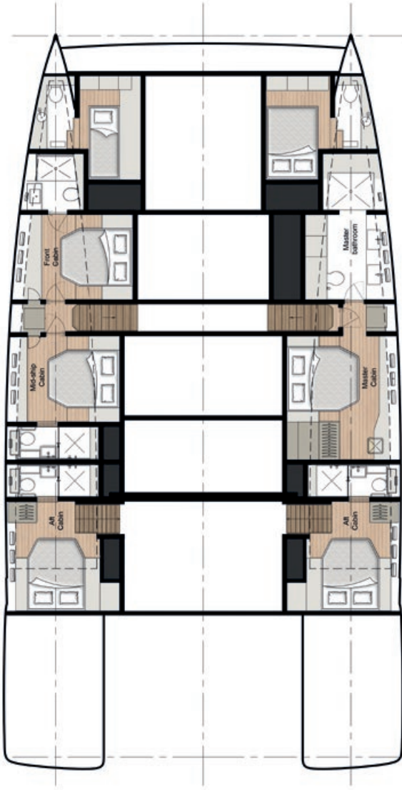
HULLS
