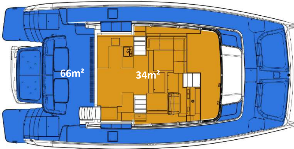
Main Deck
