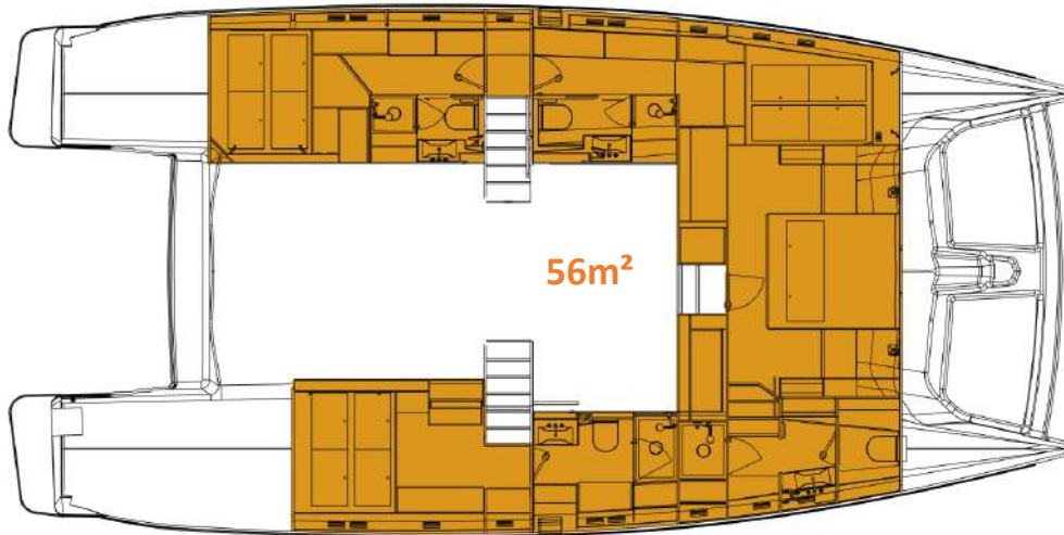
Cabin Deck - 4 Cabins / 4 Bathrooms
