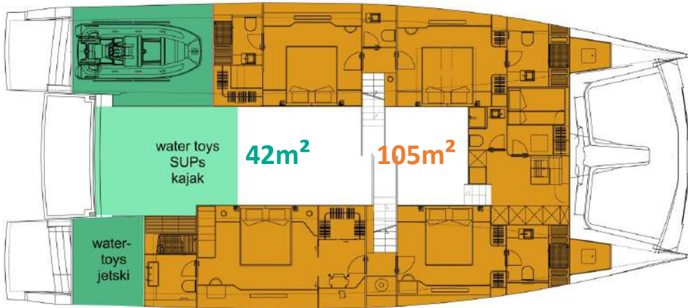
Cabin Deck
