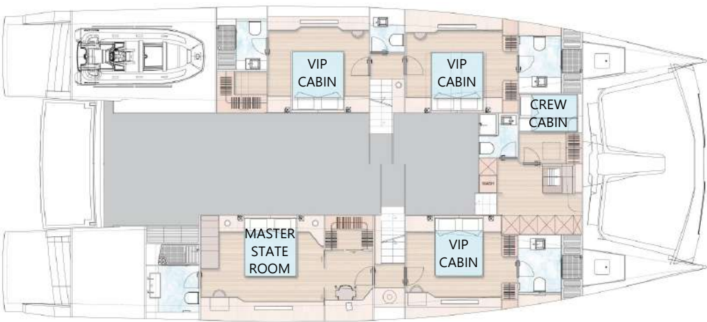
Cabin Deck - 1 Master State-Room, 3 VIP Cabins & Crew Cabin (for 2) / 5 Bathrooms
